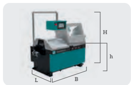
VELOX 350 AF-NC 90° B 1800 mm L 1450 mm H 1950 mm h 930 mm Kg 607
