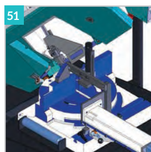
000951 BS 300-350-400 SHI
